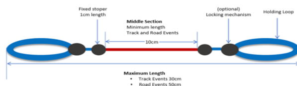
Figure 3 – Tether features
